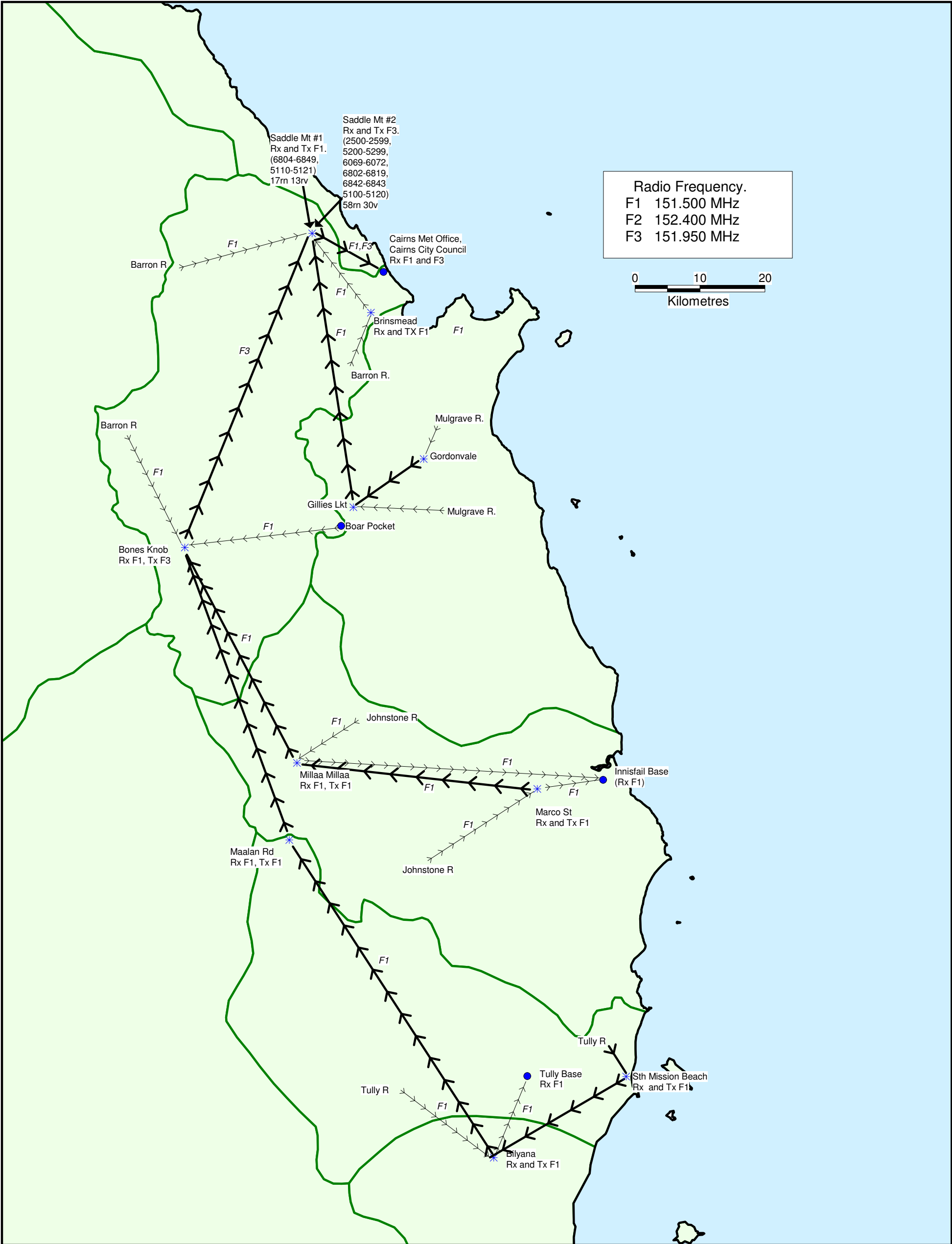
North Queensland Alert Network Repeater Network to Saddle Mt
